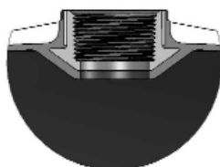
Cutaway view of top connection 1 1/4" FNPT
